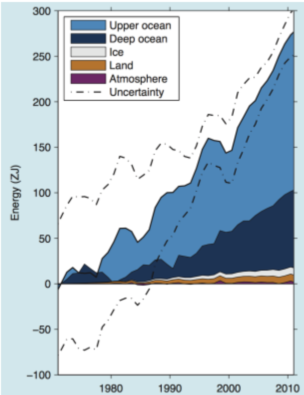
Plot of energy accumulation in ZJ (1 ZJ = 10 21 J) within distinct components of the Earth's climate system relative to 1971 and from 1971 to 2010 unless otherwise indicated.
