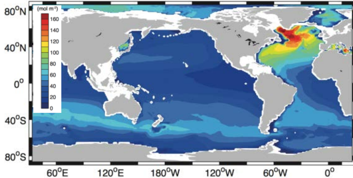
Compilation of the 2010 column inventories (mol m -2 ) of anthropogenic CO 2 : the global Ocean excluding the marginal seas
