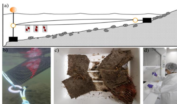
Figure 24. Field based experiments for the adsorption / desorption of metals in the marine environment; a) scheme of the deployment structure used in all sites, b) picture of the structure with bags in the marine environment, c) samples collected after one year in the water, d) extraction procedure in a class 1000 (ISO class 6) clean room.
